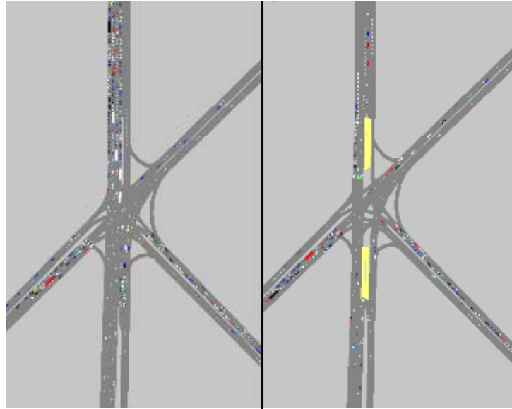
Figure 5.5. Intersection of Kapiolani Boulevard with Date and Kamoku Streets.
