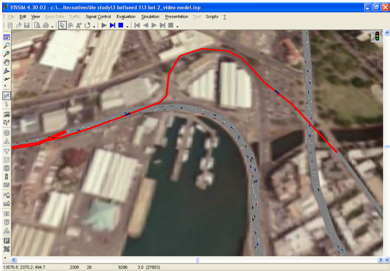
Figure 4.3. Direct connection of HOT lanes (Nimitz Viaduct) to Hotel St. Transit Mall.
