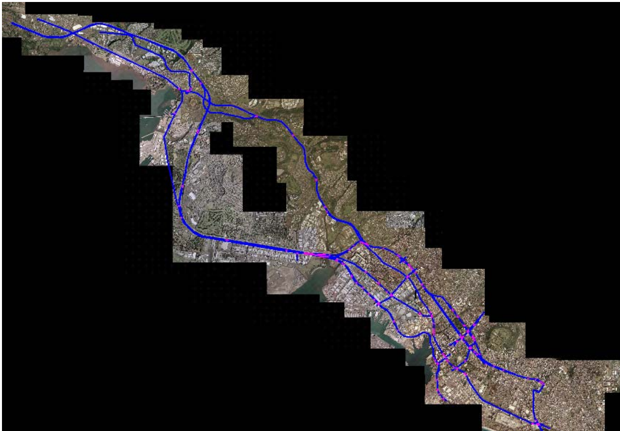
Figure 6.1. Vissim links and connectors for Honolulu's primary morning commute network.
